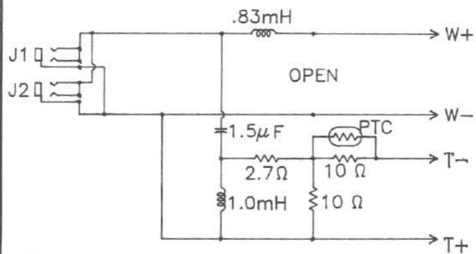
SCHEMATIC DIAGRAM
